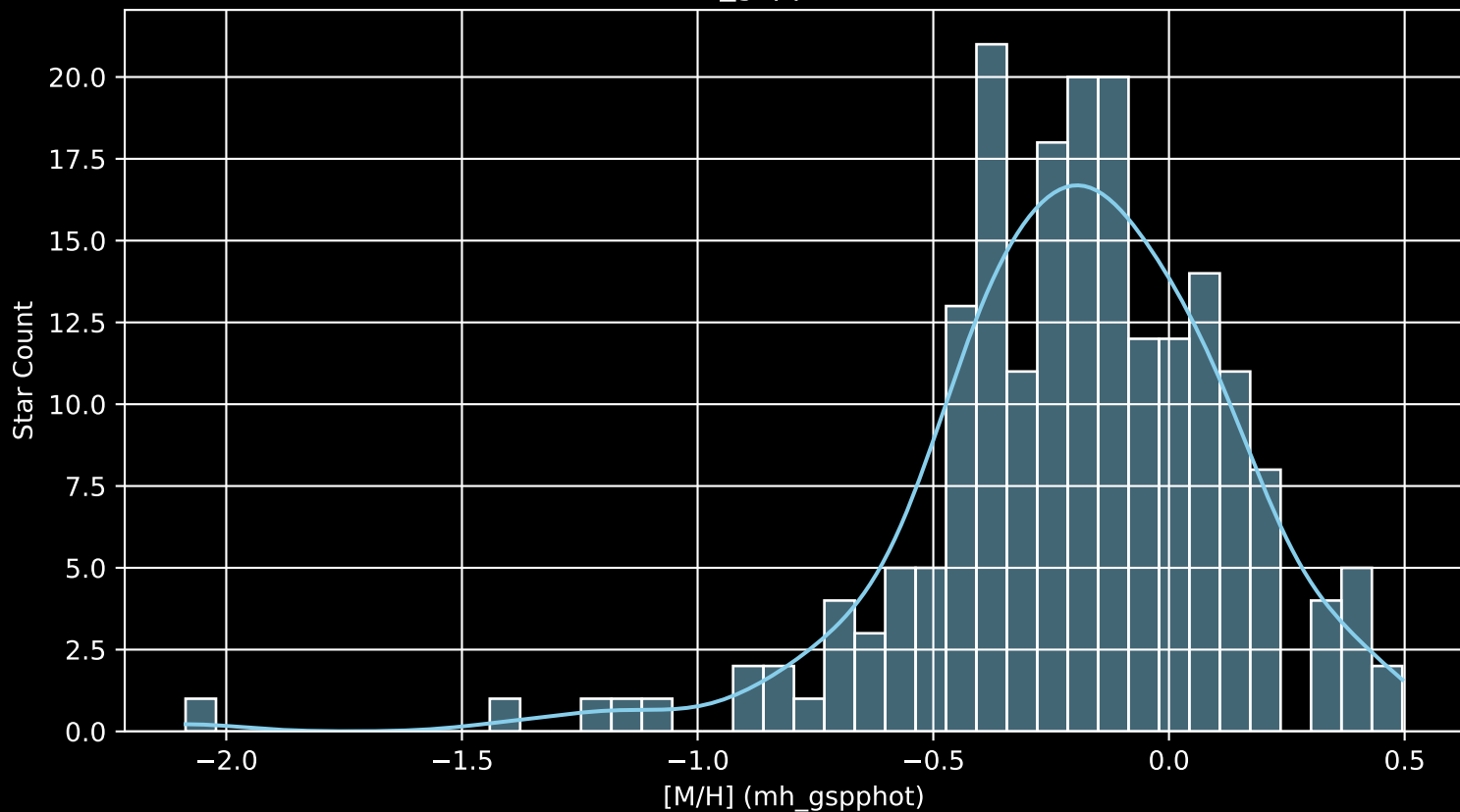
APOGEE DR17 Field: [175+58_MGA [M/H] (mh_gspphot) (n= 198)
