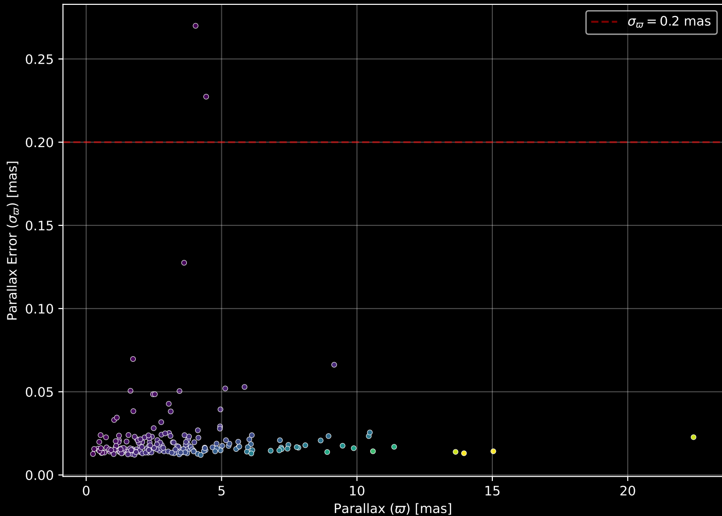
APOGEE DR17 Field: [175+58_MGA] Parallax Quality (n= 200)
