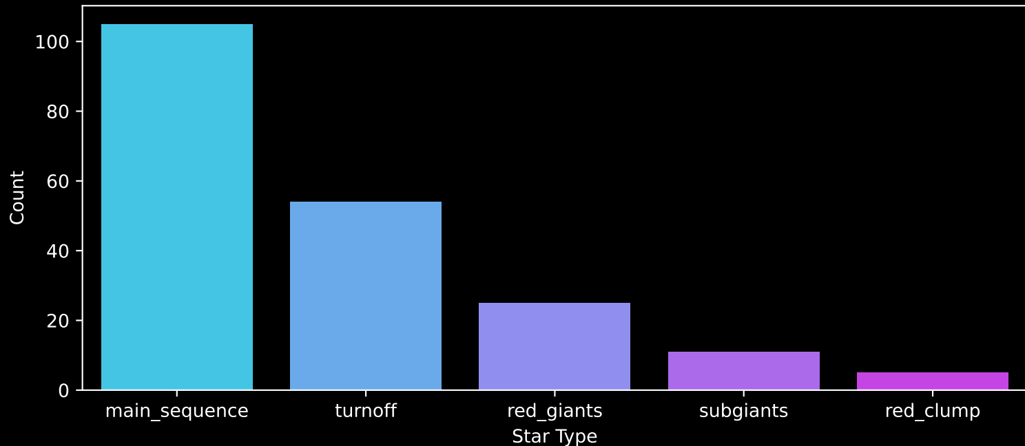
APOGEE DR17 Field: [175+58_MGA] Count plot of Star Type
