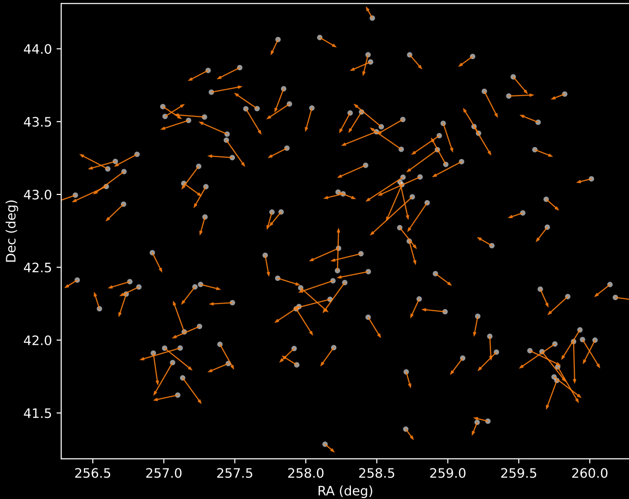
APOGEE DR17 Cluster 2 Proper Motion Vectors (n=132)
