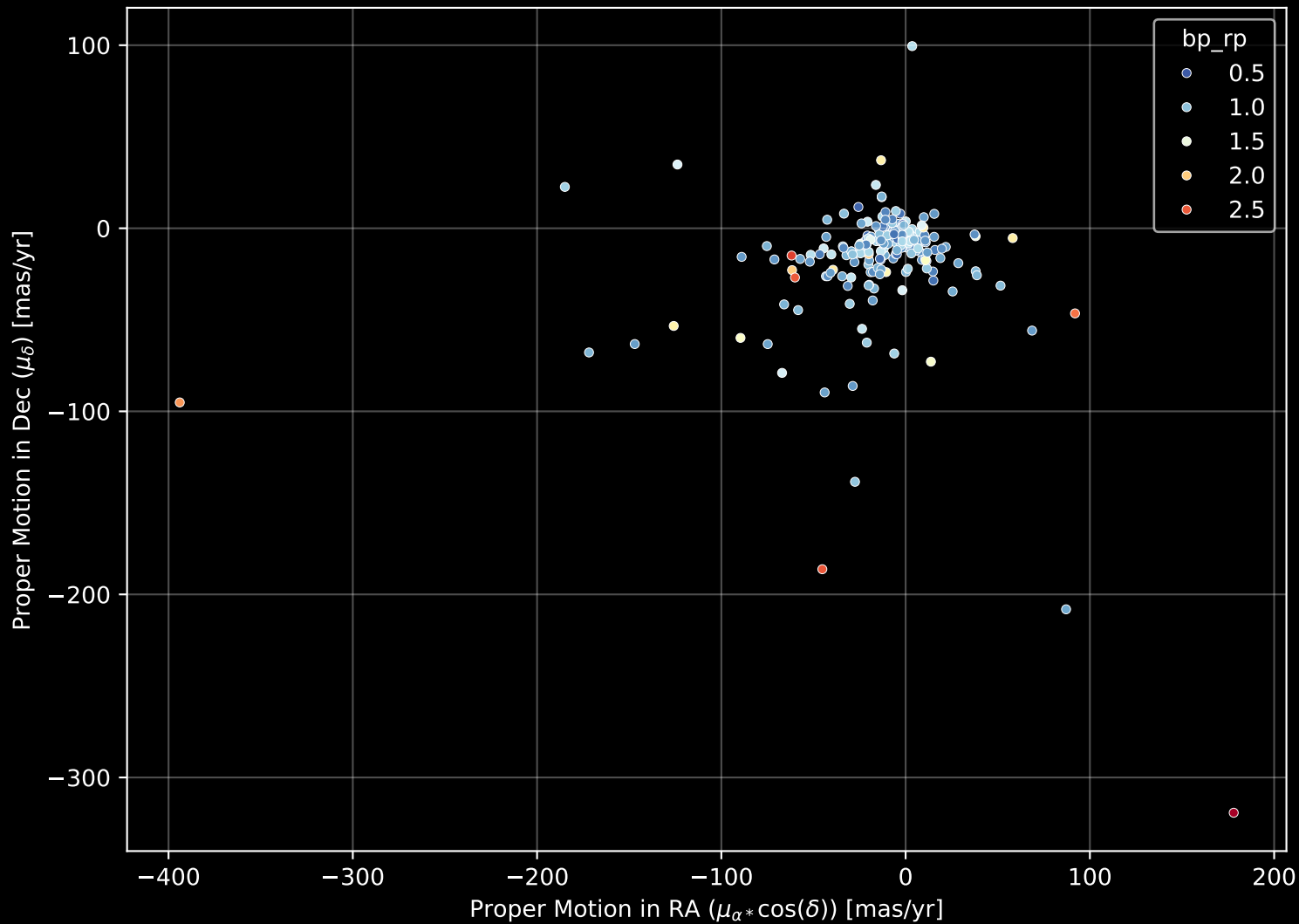
APOGEE DR17 Field: [175+58_MGA] Proper Motion Diagram (n= 200)
