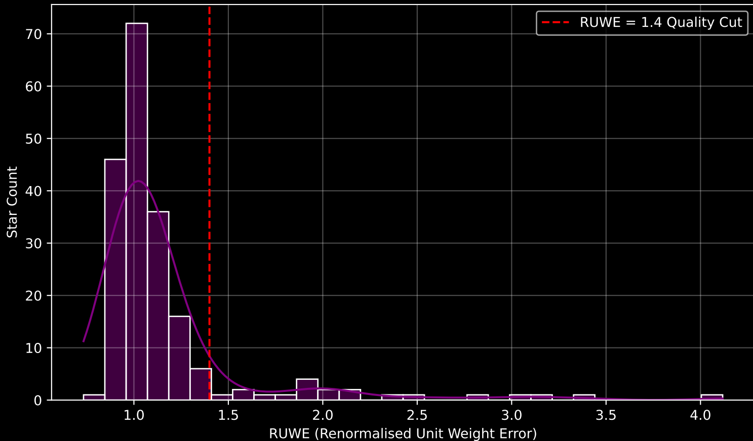
GAPOGEE DR17 Field [175+58_MGA] RUWE Distribution (n= 197)
